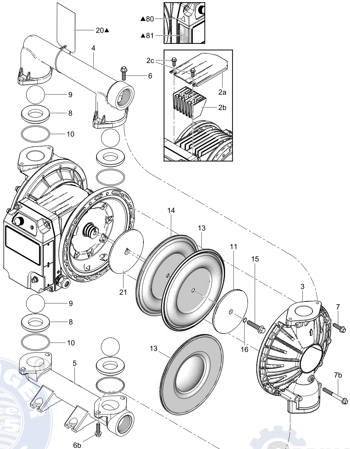
i120 (QTE) Ball Models (Aluminum model shown)
