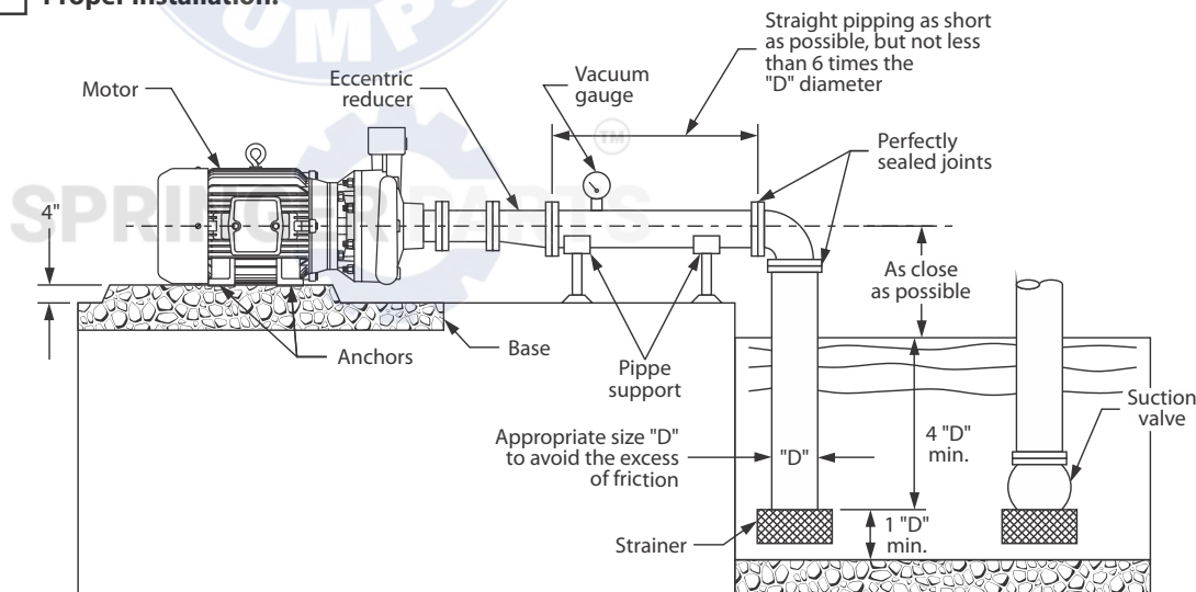
Figure 1 Proper installation.
