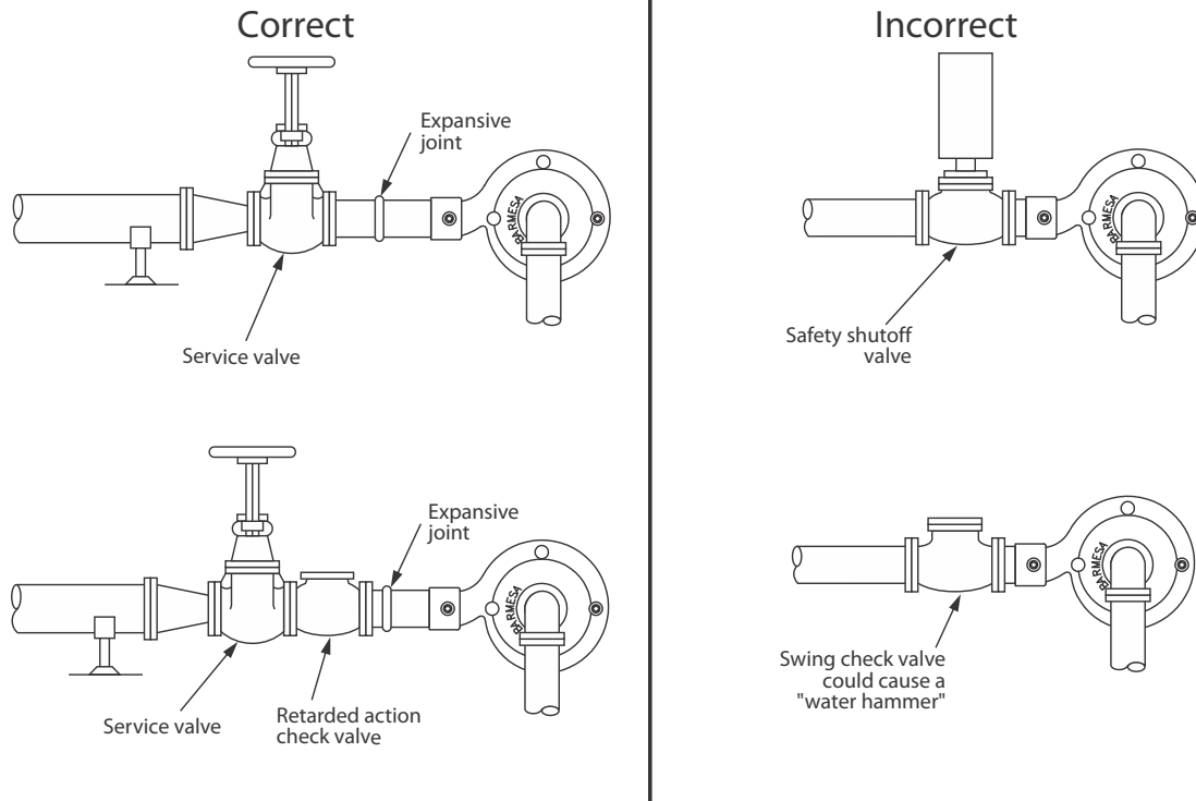
Figure 6 Discharge piping.
