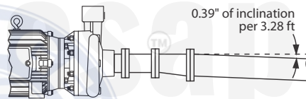
Figure 3 Inclination. Correct
