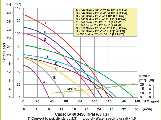
Performance of Stainless Steel Straight Centrifugal Pumps
