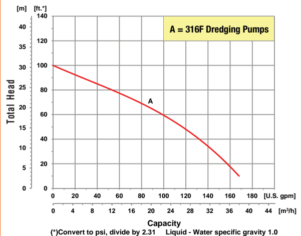
Performance of Engine Driven Dredging Pumps
