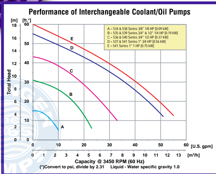
Suction Type Pump
