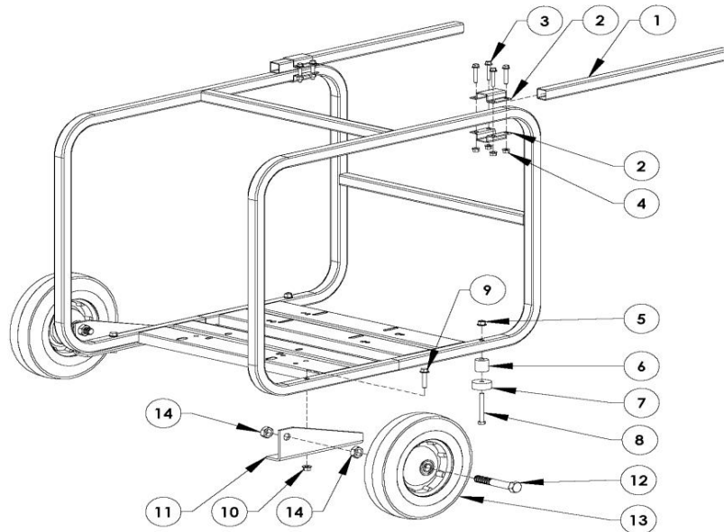
Figure 1 – Repair Parts Illustration
