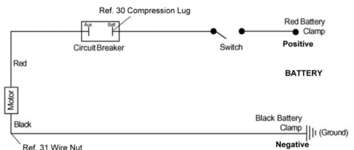
Figure 1 - Wiring Diagram
