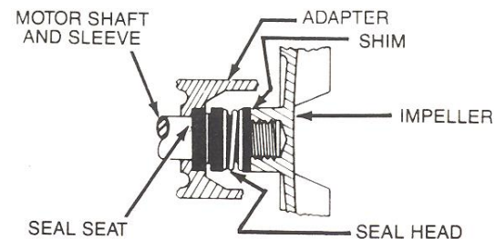
Figure 1 – Mechanical Seal
